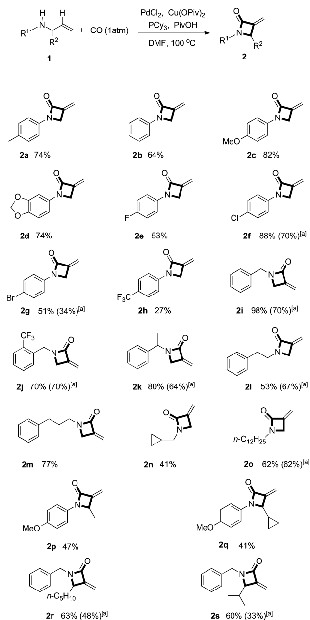
Scheme 3. Carbonylation of various N -allyl amines to give \alpha -methylene- \beta -lactams. Reaction conditions: 100 °C, N -allylamine (0.2 mmol), PdCl 2 (10 mol %), PCy 3 (20 mol %), Cu(OPiv) 2 (0.4 mmol), PivOH (0.4 mmol), CO (1 atm), DMF (2 mL), 1–24 h. Yield of isolated 2 is given. [a] The reactions were carried out in an autoclave.
